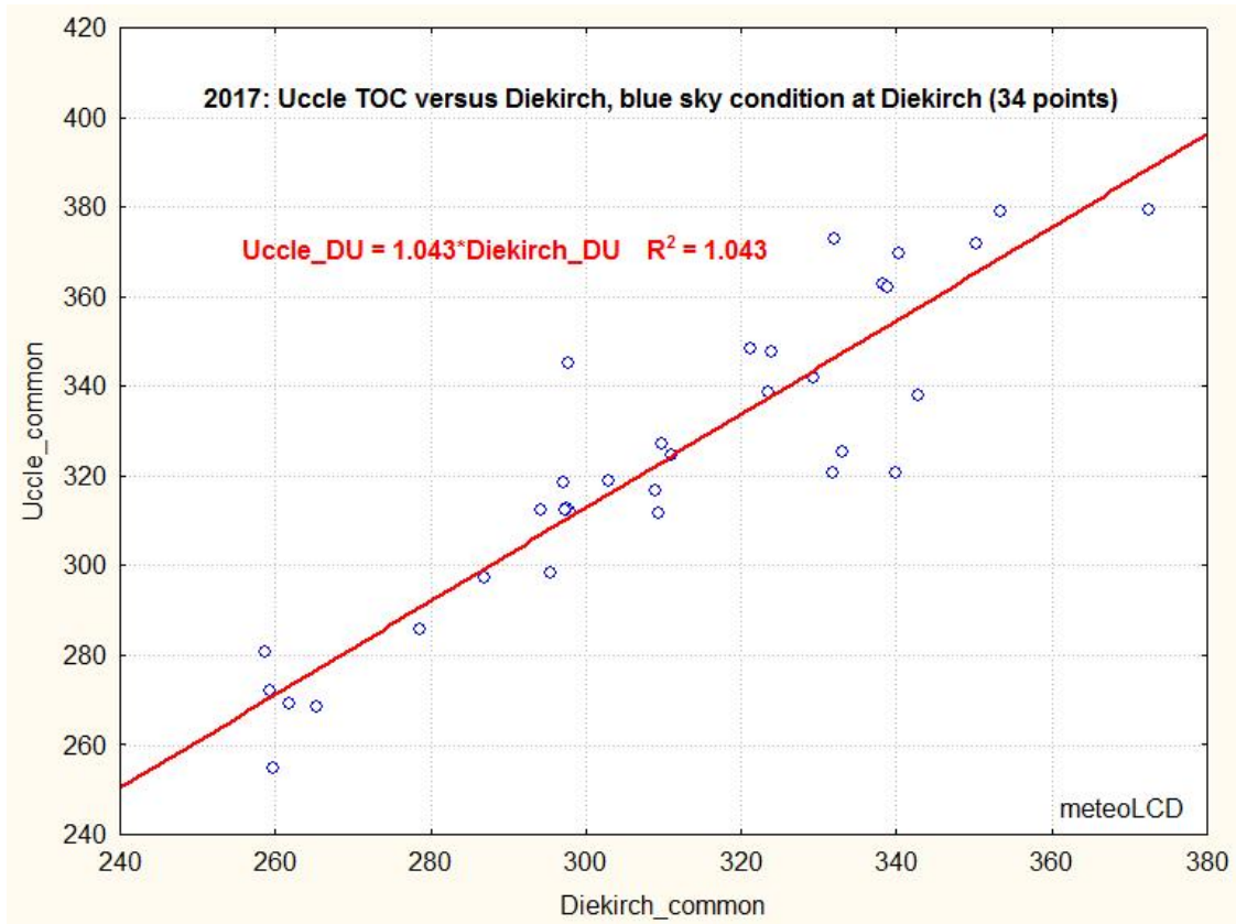
Fig.5. Uccle Brewer#178 versus same day Diekirch measurements, blue sky only
