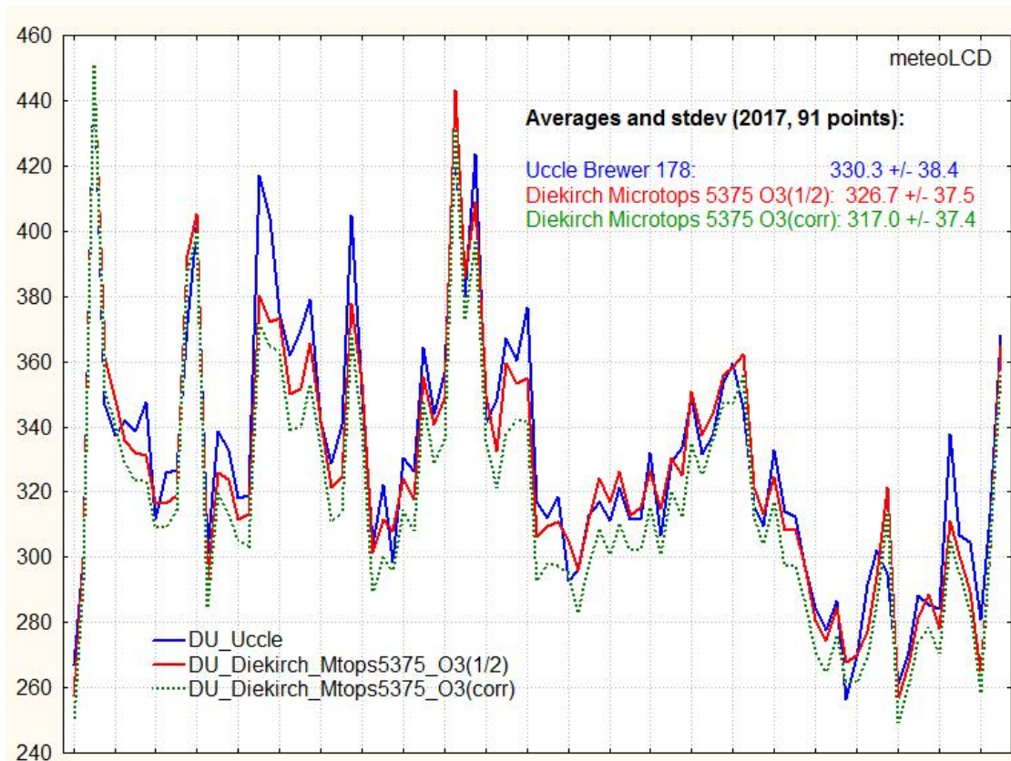
Fig.6. Uccle and Microtops #5375 channel 0 and channel 1 readings.
