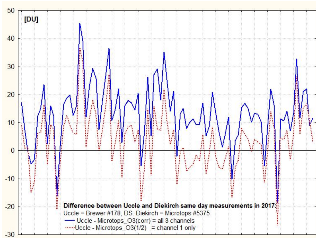
Fig.7. Difference of the two readings O3(corr) and O3(1/2).and the Uccle Brewer.
