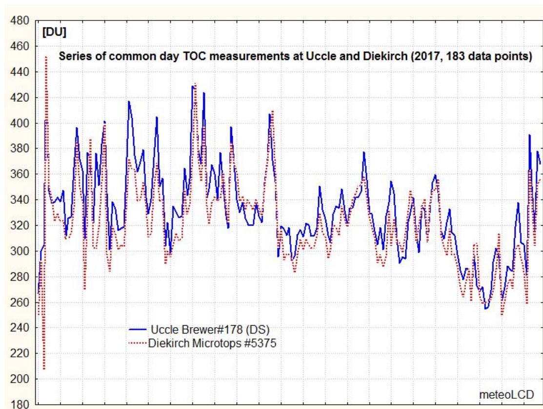
Fig.1. Uccle Brewer #178 and same day Diekirch TOC (DS only).
