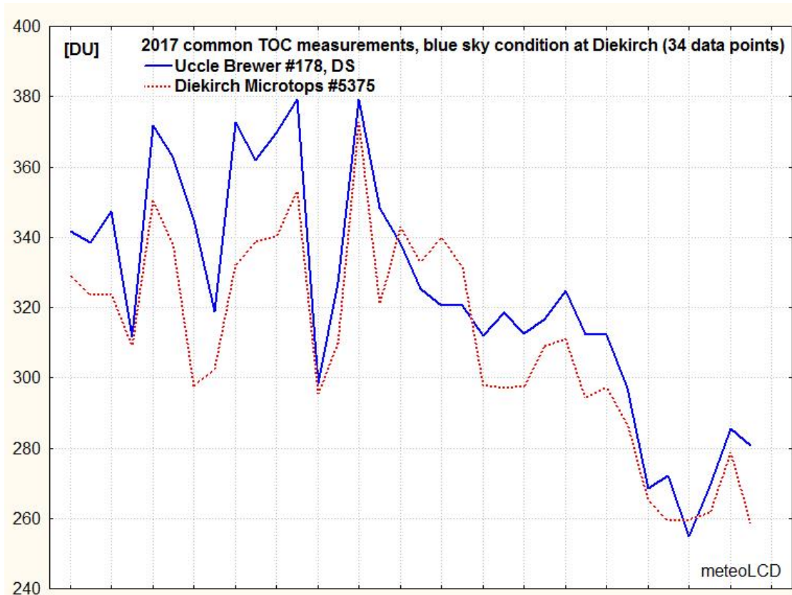
Fig.4. Uccle Brewer #178 DS and same day Diekirch TOC (blue sky only).
